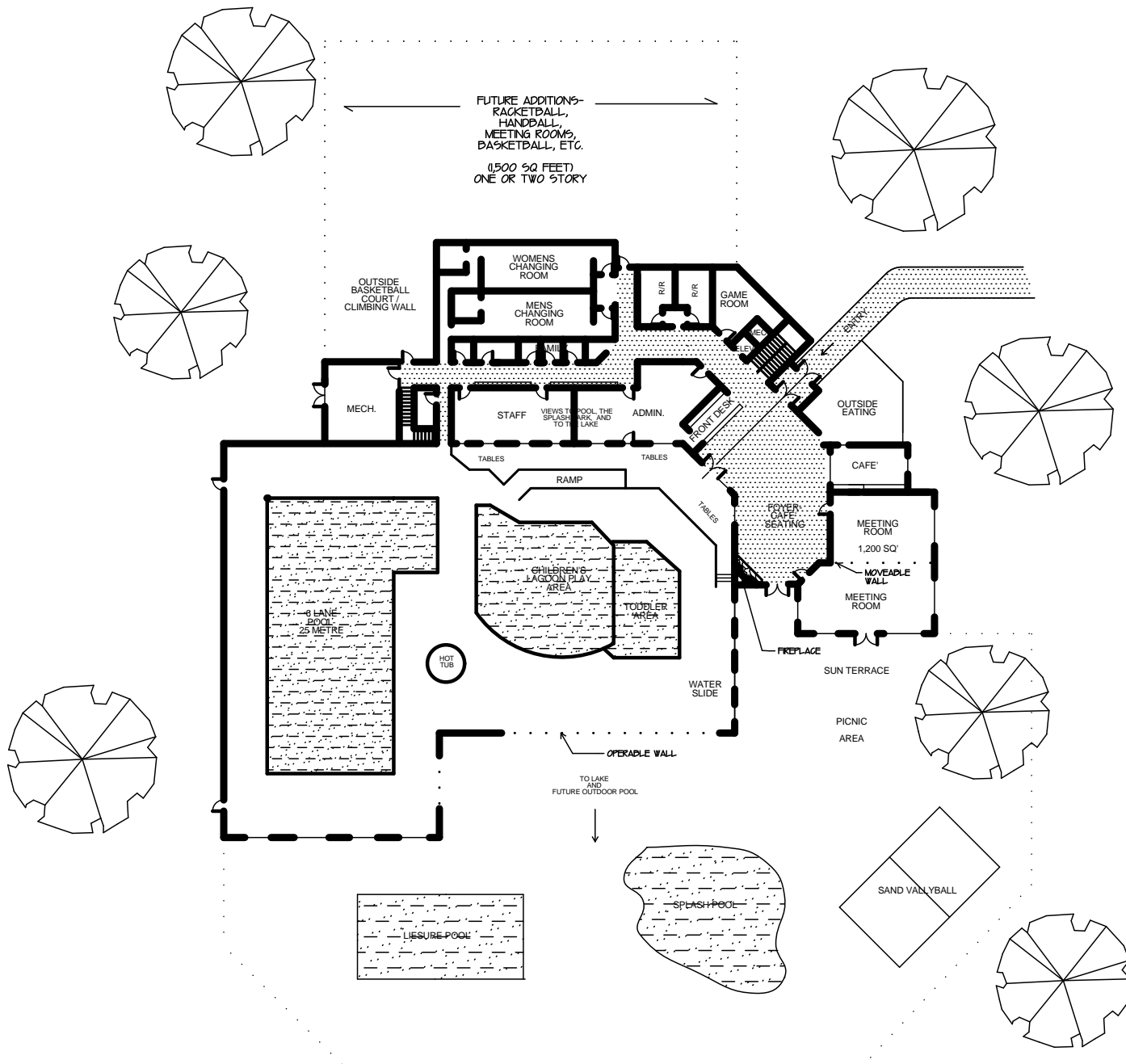
◆ SCHEMATIC PLAN - MAIN FLOOR 20,000 SQ'
